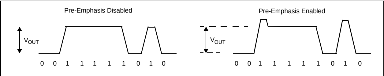
Figure 5. Pre-Emphasis Diagram
