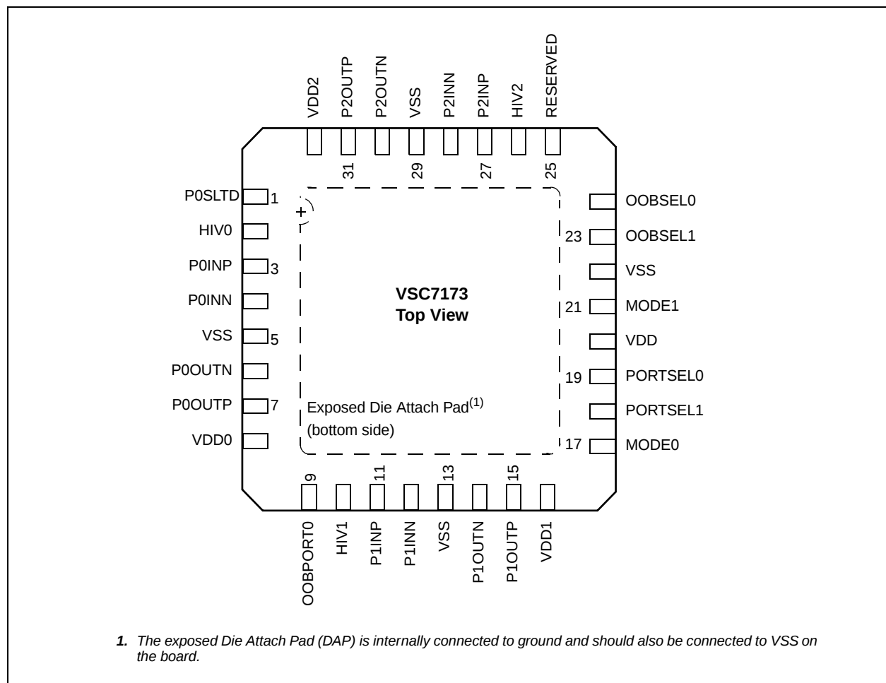
Figure 9. Pin Diagram
